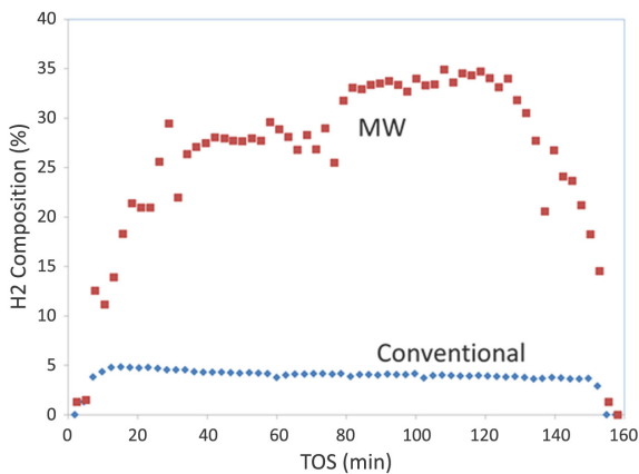
Figure 3: Coal steam gasification.
