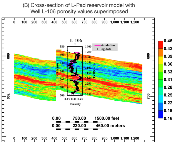
Figure 3. Modeling results for the Prudhoe Bay Unit, L-Pad reservoir, North Slope Alaska. (A) 3D model of the L-Pad reservoir geology showing sedimentary layering, faulting, and porosity. (B) Cross-section of the L-Pad reservoir model with Well L-106 porosity curves superimposed– including simulated log curve (in red) and measured log data (black dots).
