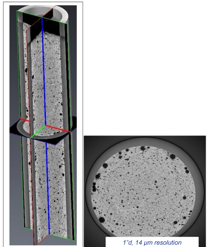
Figure 1. 3D CT scans of a 1-inch cement core.
