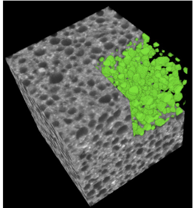
Figure 4. Segmented portion of 30 percent quality atmospherically generated foamed cement scanned with NETL's high-resolution industrial CT scanner. Cement displays fairly homogeneous distribution of voids.
