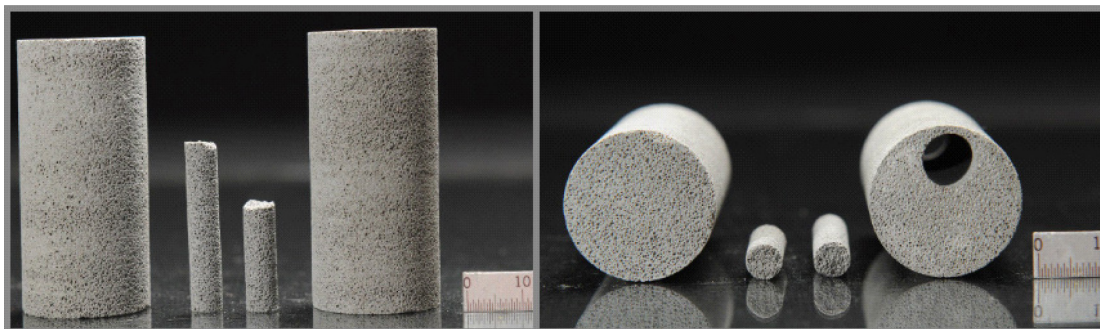
Figure 2. Lab-generated atmospheric 40 percent quality foamed-cement samples.
