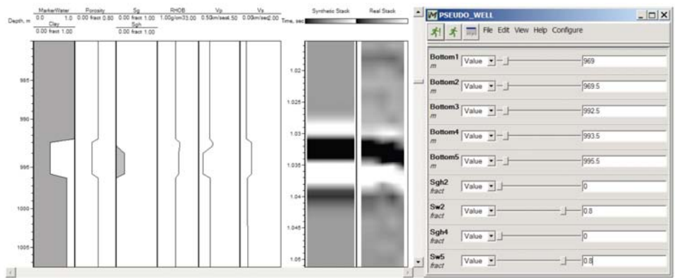
Figure 7: Same as Figure 6 but without hydrate and with free gas. Zooming on the main seismic event.
