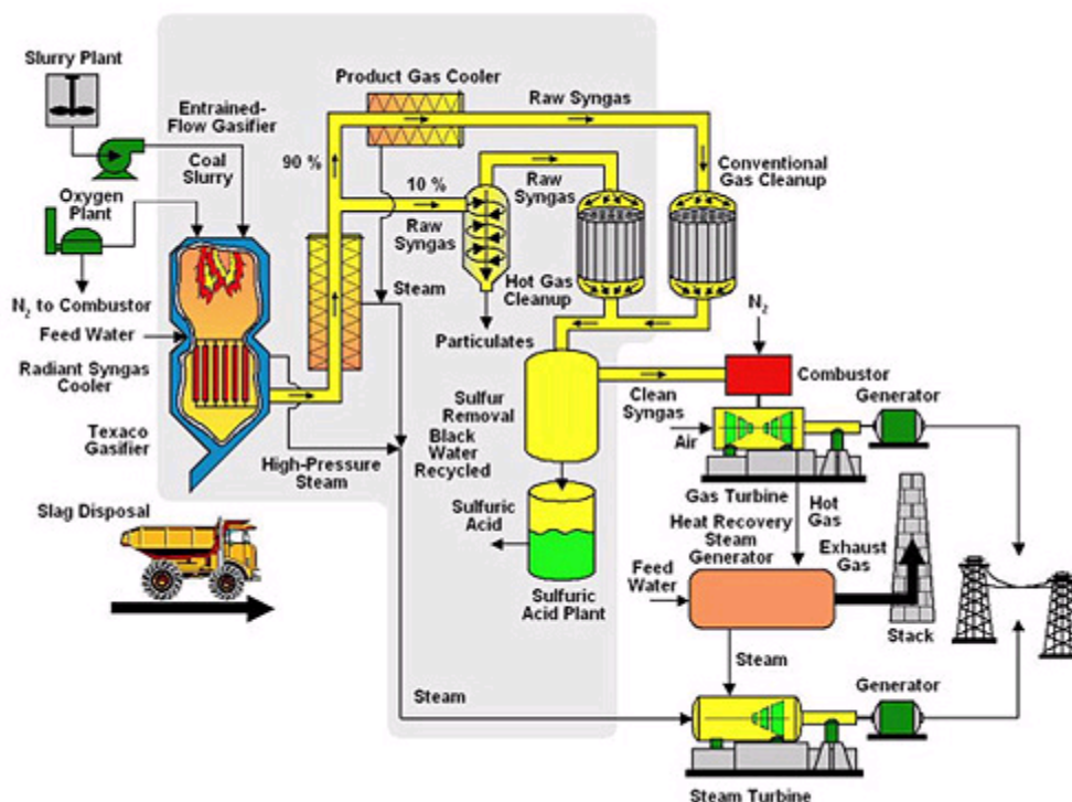
Figure 1.1—IGCC Process 7
