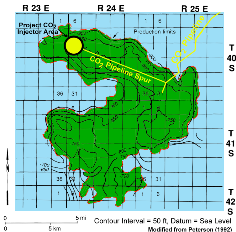
Figure 4. Structure map of top of the Desert Creek zone.
