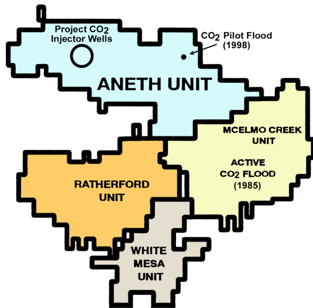
Figure 2. Units within the greater Aneth field.
