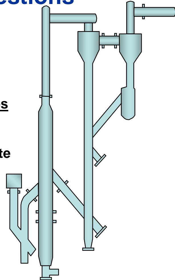
285 MW Commercial gasifier
