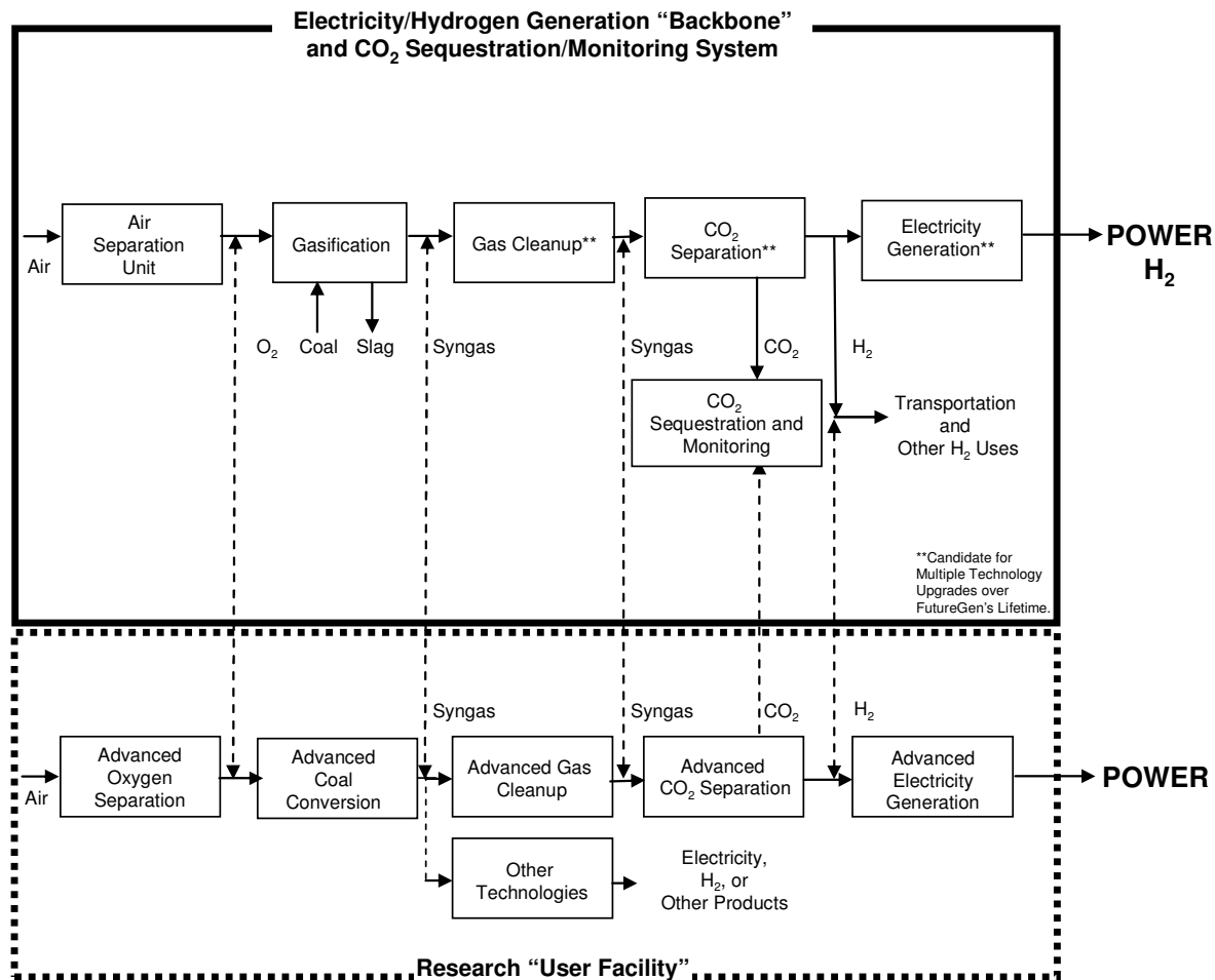
Figure S-17. FutureGen Power Plant Overview
