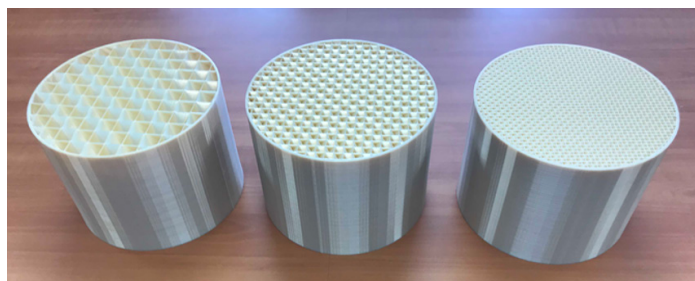
3D printed intensified packings for enhanced solvent-based CO 2 capture
