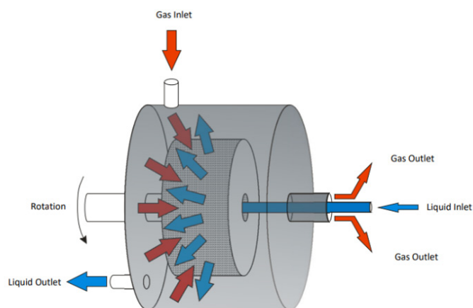
Process intensification using a rotating packed bed absorber
