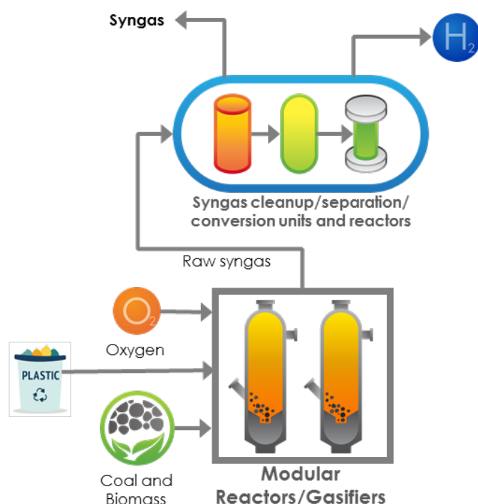
FIGURE 1. A Gasification Production Key Technology—Process Intensification for Hydrogen and Syngas Production
