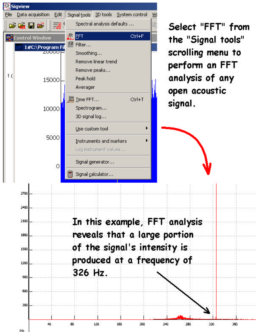
Figure 33: Sample result of Signal View's FFT analysis.
