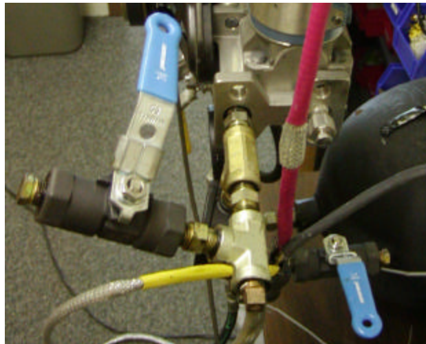
Figure 8: Photograph of OASC installed on PAMP. Each of the blue handled valves is an OASC with a different frequency-pressure curve.
