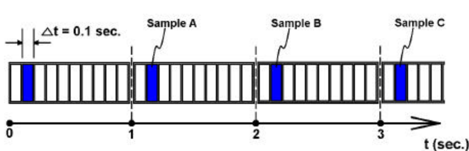
Figure 10: 0.1-second acoustic signal sampling occurs at 1-second intervals.
