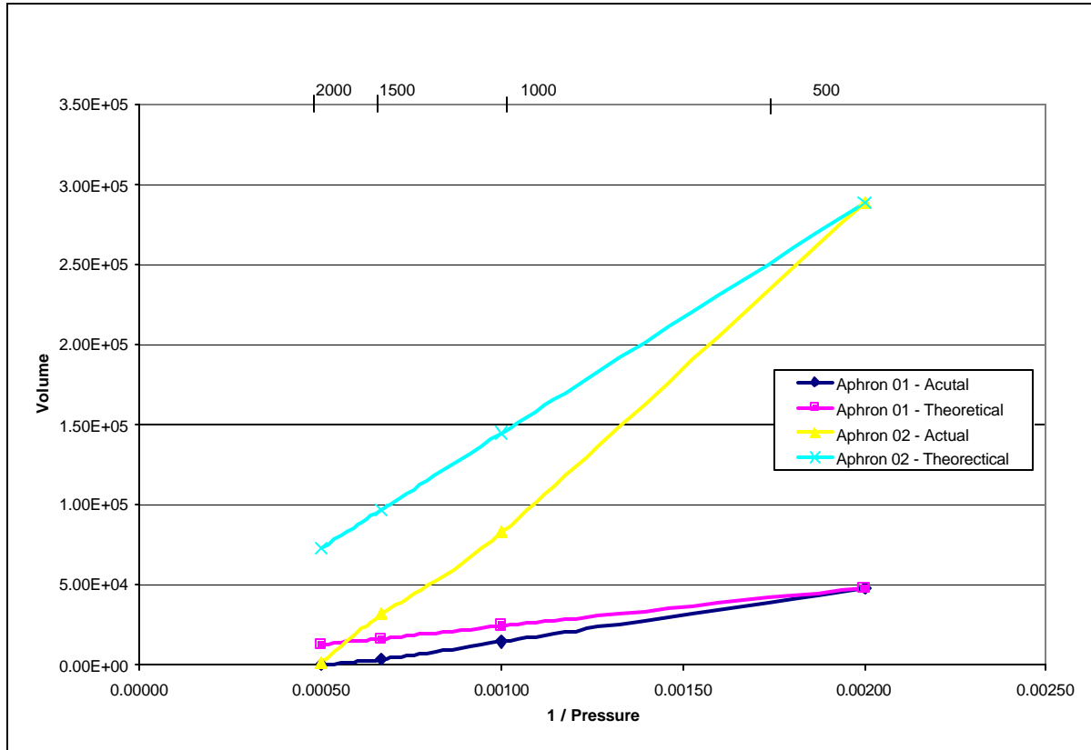
Figure 5. Effect of Pressure on Size of Aphrons in Transparent APHRON ICS Mud
