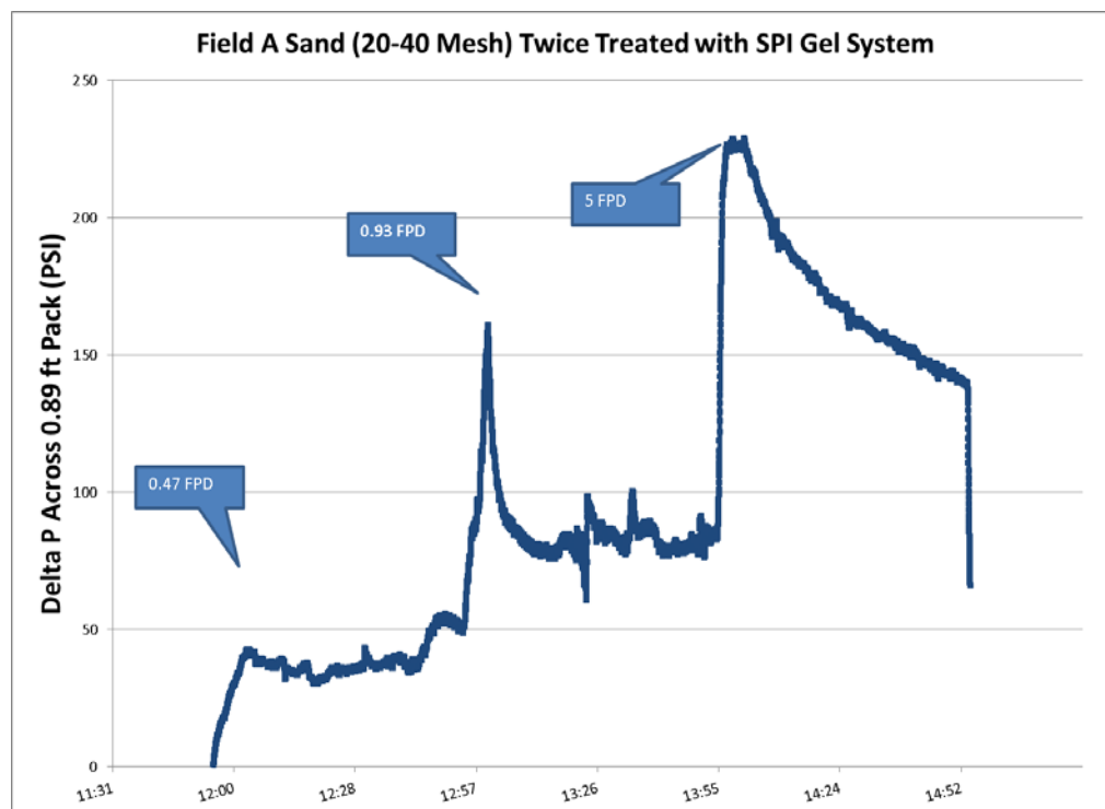
Figure 23. Water Injectivity Tests in a Sandpack with Field A sand material after two SPI Treatments
