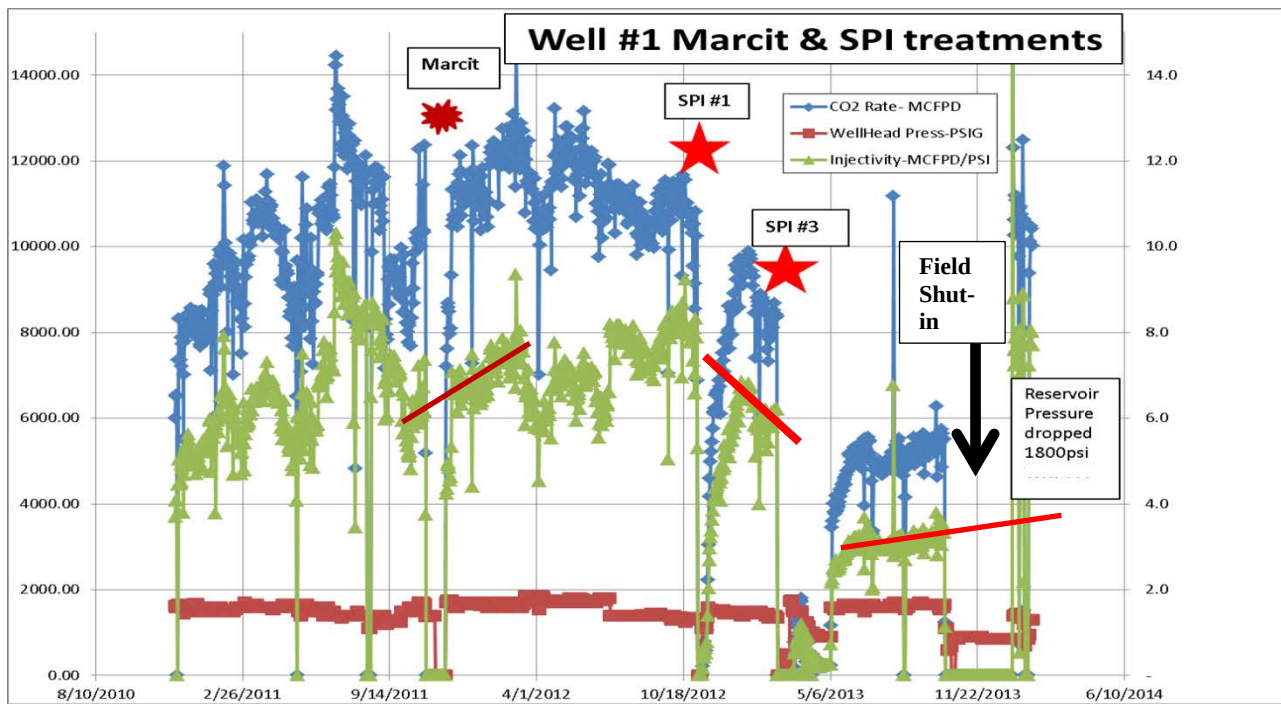
Figure 57. Field A, Well #1 Injection History Plot showing both Marcit™ and SPI gel Treatments
