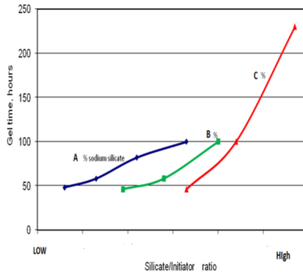
Figure 5. SPI Gel Time at 40°C versus Silicate/Initiator wt /wt Ratio
