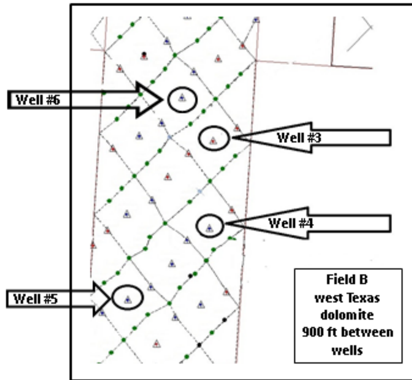
Figure 49. Field B Map showing Location of all SPI Treated Injection Wells
