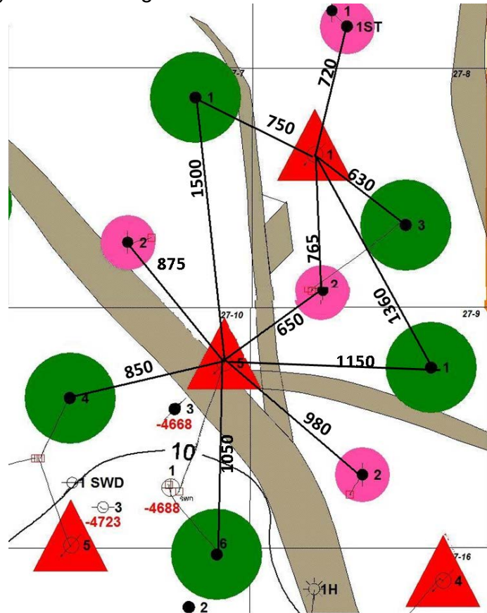
Figure 35. Field A Map showing Distances between Wells in one pattern
