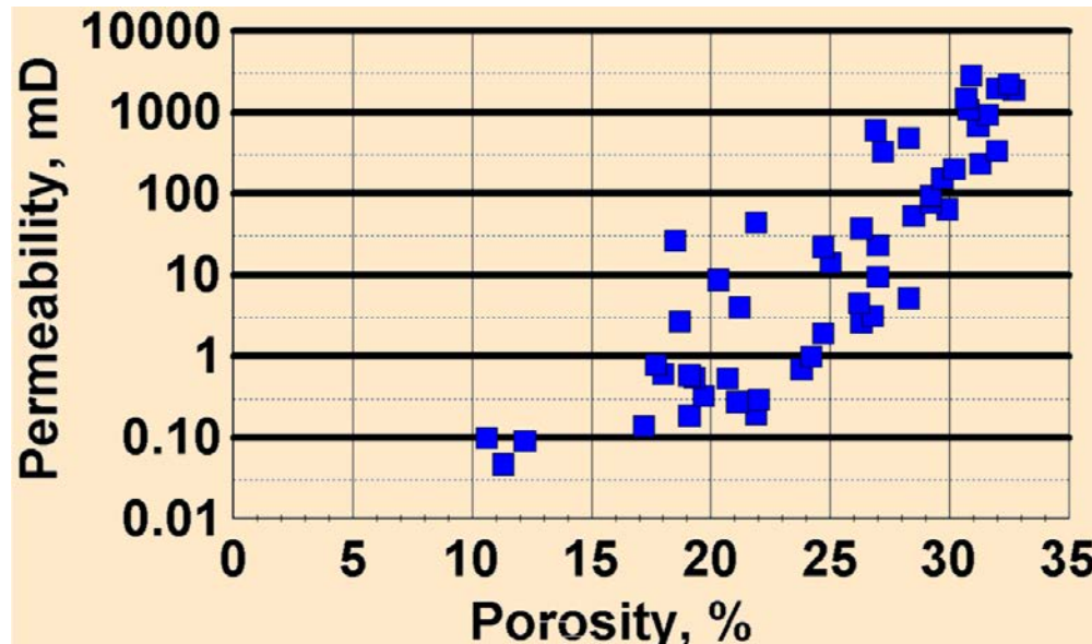
Figure 29. Field A Permeability versus Porosity from Core Analysis
