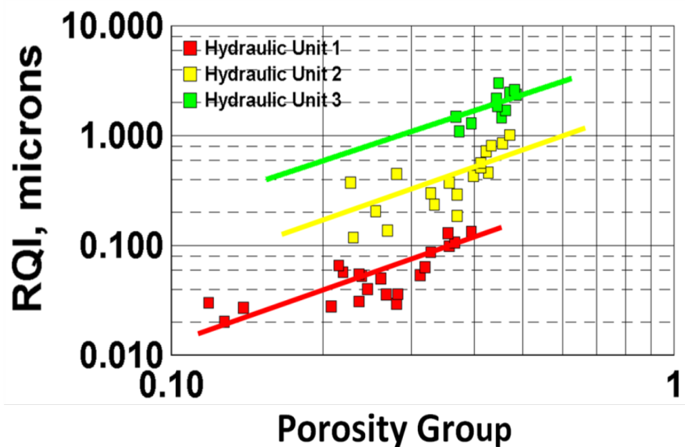
Figure 30. Plot Field A Reservoir Quality Index to Identify Hydraulic Units
