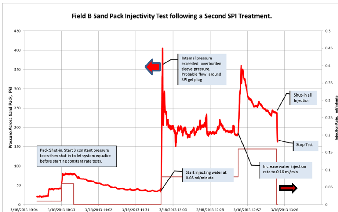
Figure 26. Water Injectivity re-Test of Field B Dolomite Sand Pack with early Constant Pressure Period before Constant Rate, following 2 nd SPI Treatment.
