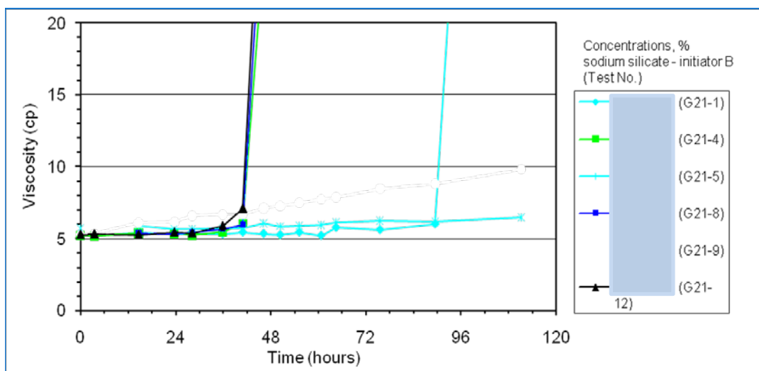
Figure 3. Previous SBIR Phase I Project Viscosity Tests showing Gel Time.
