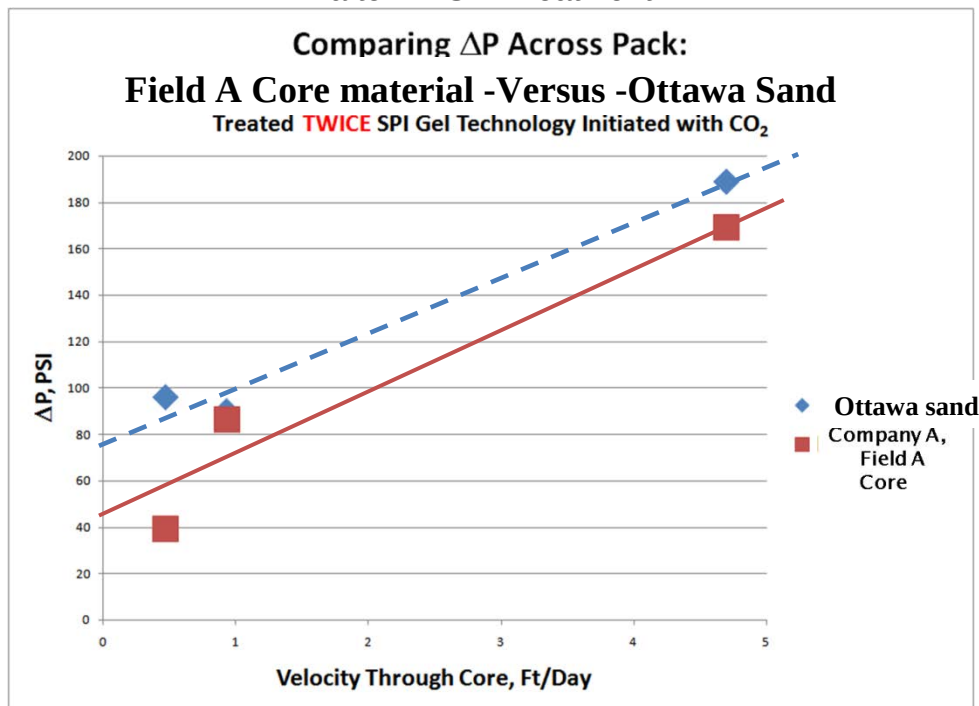
Figure 25. Field A Sandstone and Ottawa Sand Pack Water Injectivity Tests after 2 nd SPI Treatment
