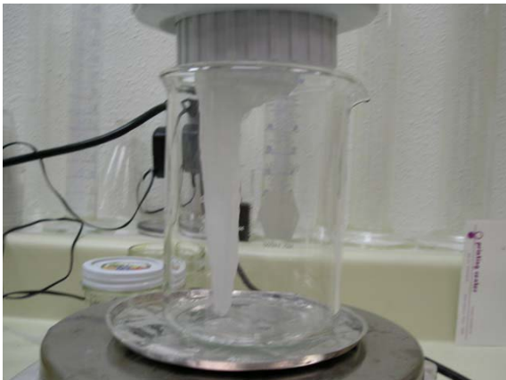
Figure 6. PAM cross-linked with Aluminum-Citrate tested through BGST
