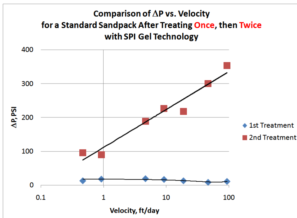
Figure 22. Sand Pack (with Ottawa sand) Water Injectivity Tests after SPI Treatments
