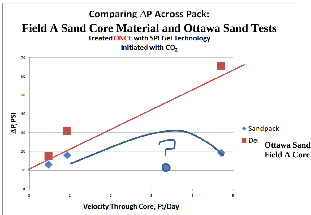
Figure 24. Field A Sandstone and Ottawa Sand Pack Water Injectivity Tests after 1 st SPI Treatment
