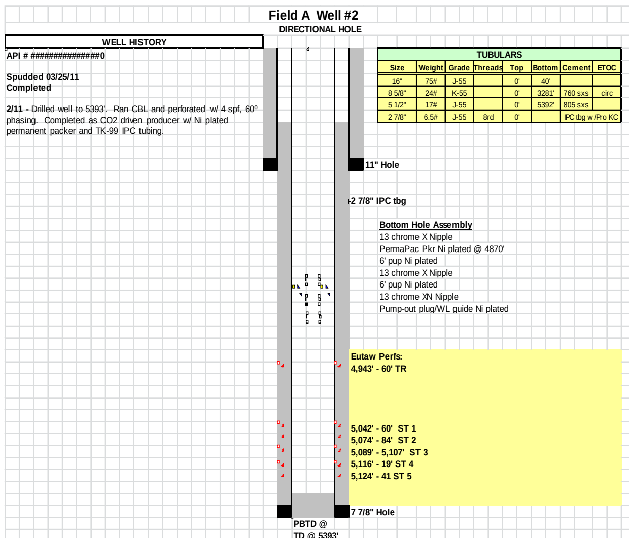
Figure 46. Wellbore Schematic for Field A, Well #2 Producer
