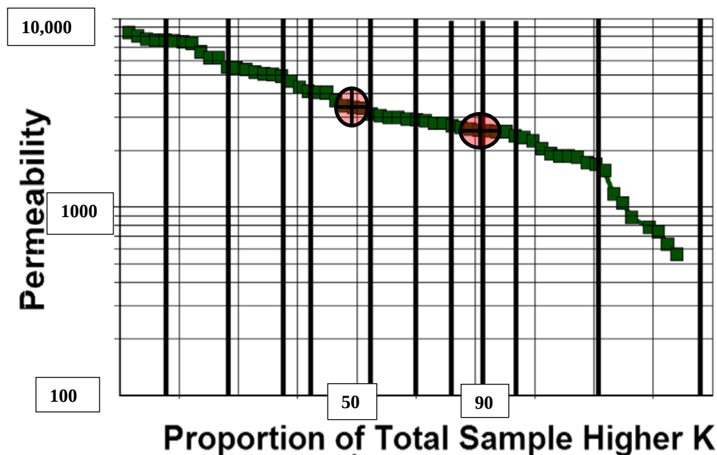
Figure 32. Plot of Field A Permeability Distribution
