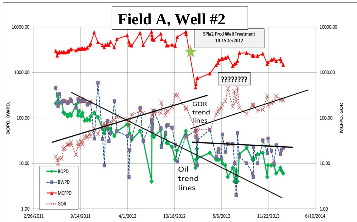
Figure 48. Field A, Well #2 Production History (with SPI2 shown as a green star).
