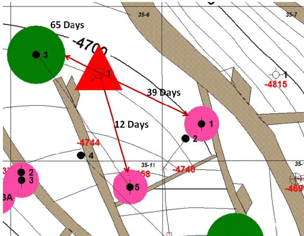
Figure 34. Field A Structure Map of one pattern with Response Times shown. Red triangles=injectors;Round=producers with different colors indicating different zones.
