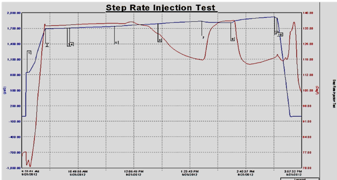
Figure 47. Field A, Well #2's (Production Well) pre-SPI Treatment Water Step Rate Test with bottom-hole pressure/ temperature bomb/ sensor.
