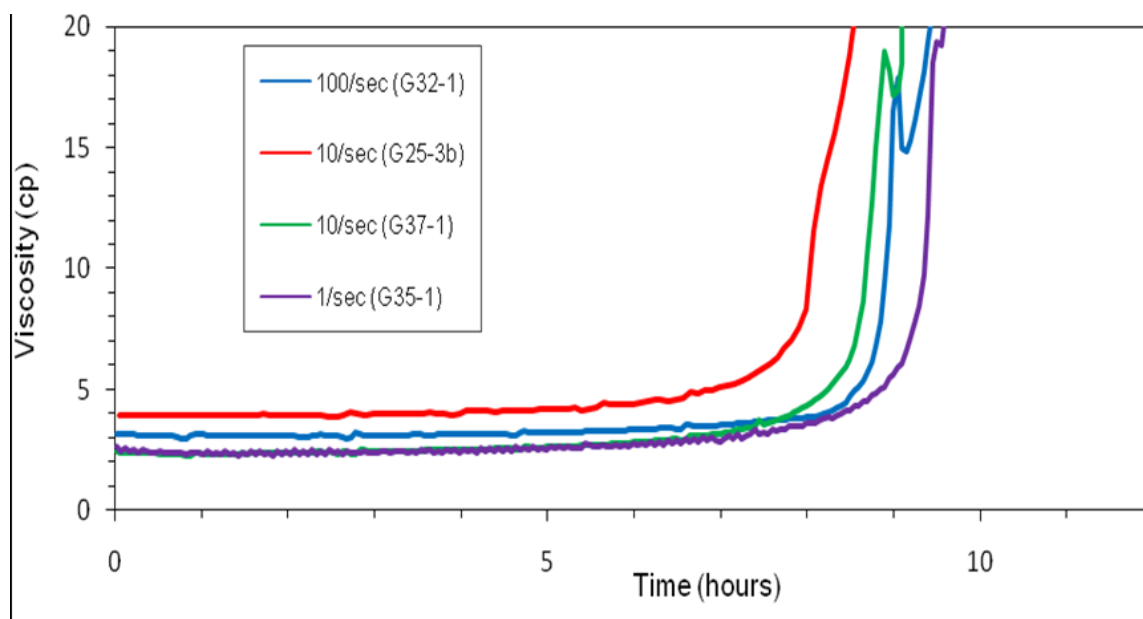
Figure 4. Prior project testing showing Viscosity of low SPI concentration (1/3 of currently field systems) solutions at 40°C (104°F) in the Brookfield Viscometer from mix time to gelation.
