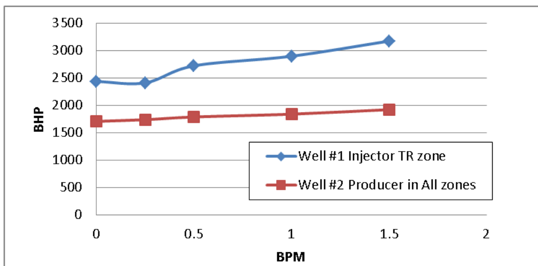
Figure 37. Comparison of Field A's Well #1 and Well #2 Water Injectivities
