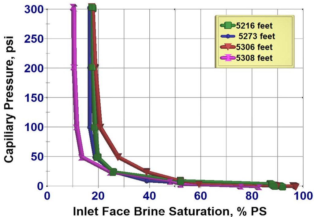
Figure 33. Plot of Field A Capillary Pressure by Depth and Brine Saturation
