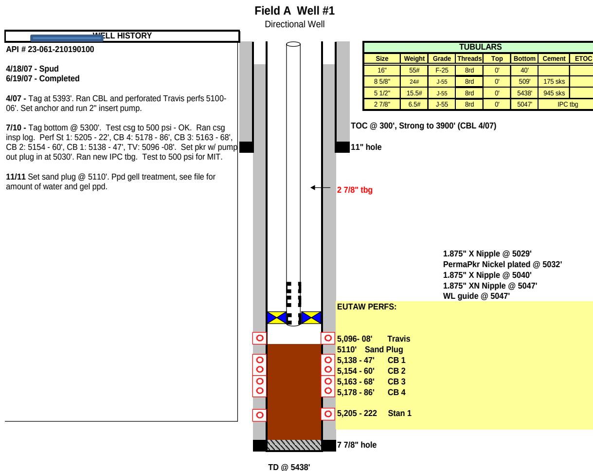
Figure 38. Wellbore Schematic for Field A, Well #1 Injector
