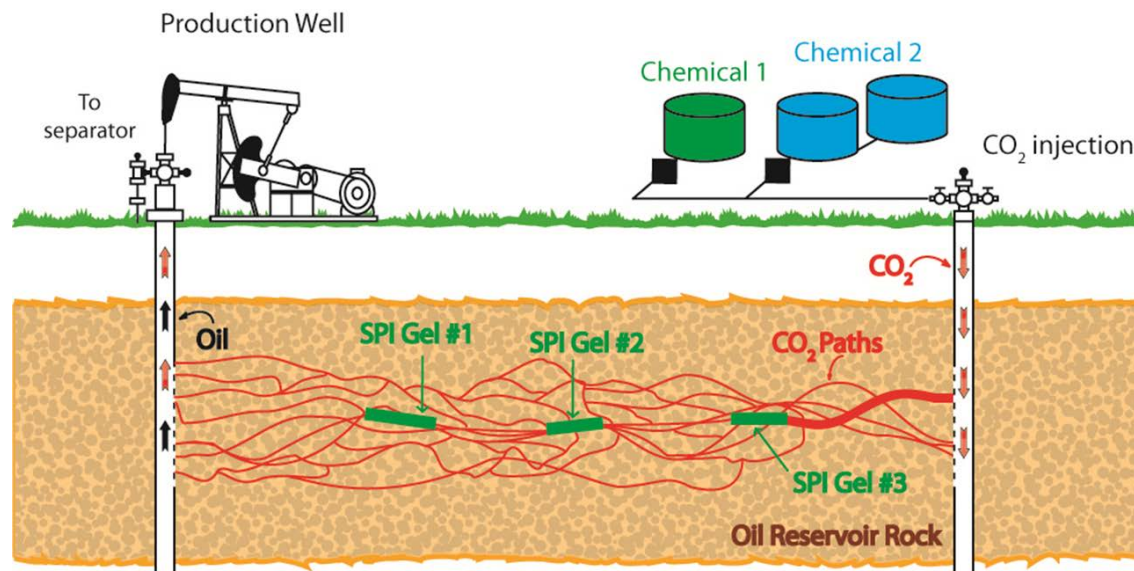
Figure 10. Schematic of Multiple, Smaller SPI Treatments in a Simplified CO 2 Flood
