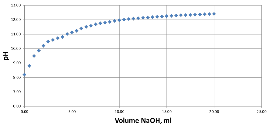
Figure 16. Titration with 0.1M NaOH into 100 grams of Field A Brine
