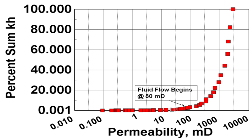
Figure 31. Plot Field A Core Permeability versus % perm-height (purpose- to determine where fluid begins to flow= 80md)
