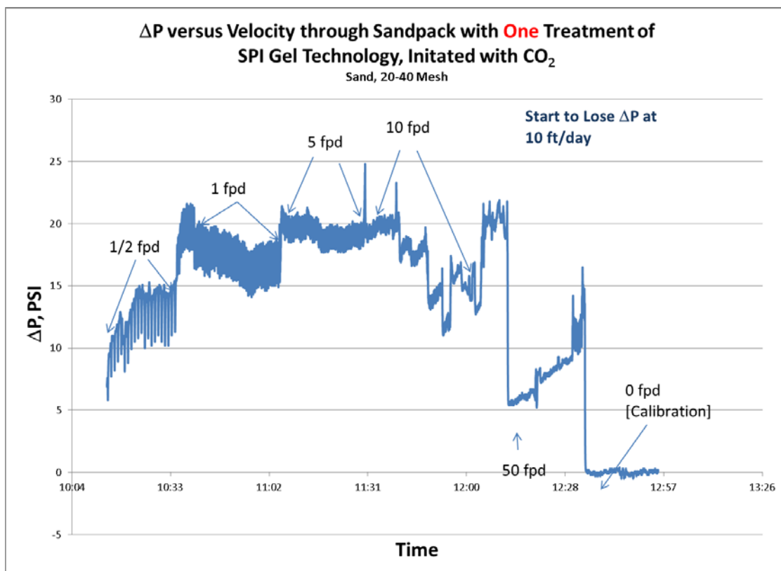
Figure 20. Sand Pack with 20-40 Mesh Ottawa Sand during Water Injectivity Tests after one SPI Treatment.
