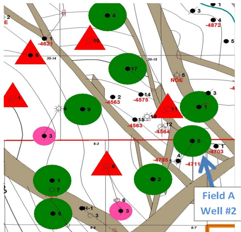
Figure 45. Field A Structure Map showing Well #2's location.
