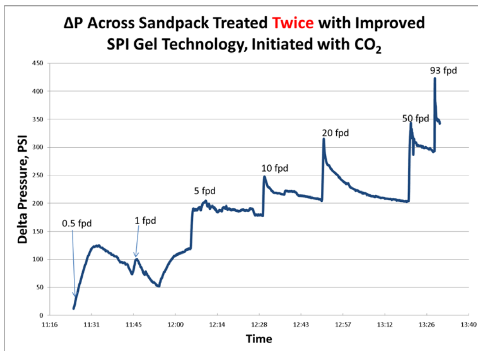
Figure 21. Sand Pack with Ottawa 20-40 Mesh sand during Water Injectivity Tests after a second SPI Treatment
