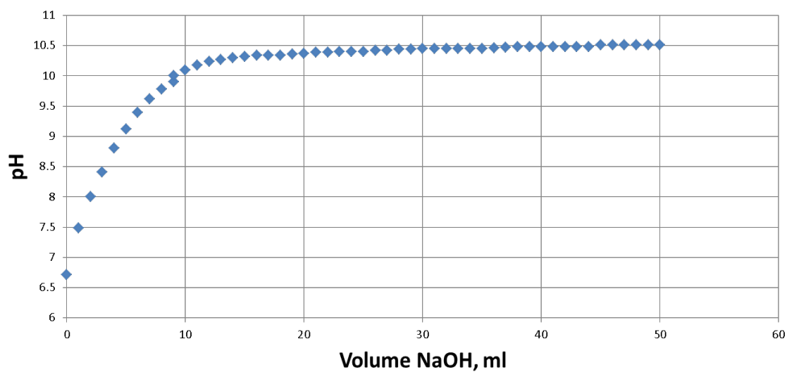
Figure 17. Titration with 0.1M NaOH into 250 ml Deionized Water with 25 grams of Field A's Crushed Sandstone
