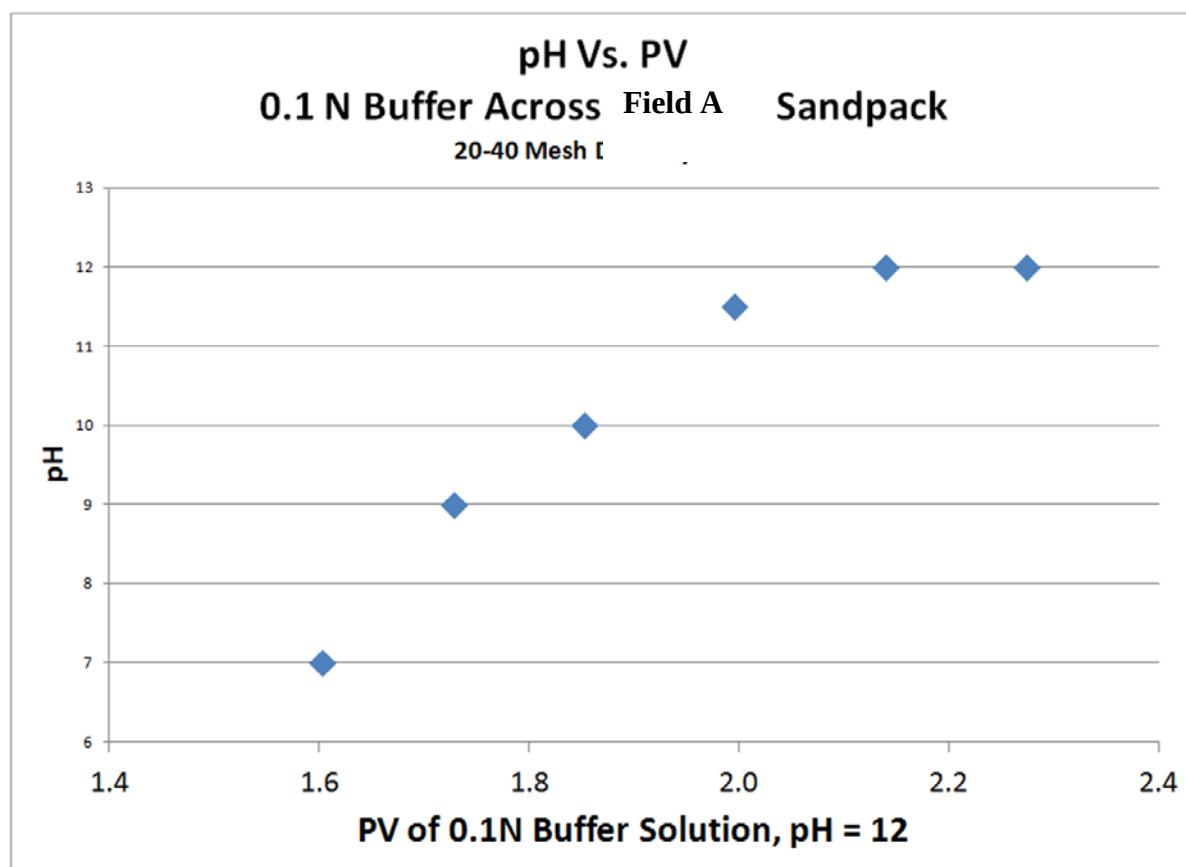
Figure 18. Titration of 0.1 N NaOH across a Sandpack with Field A sand material.
