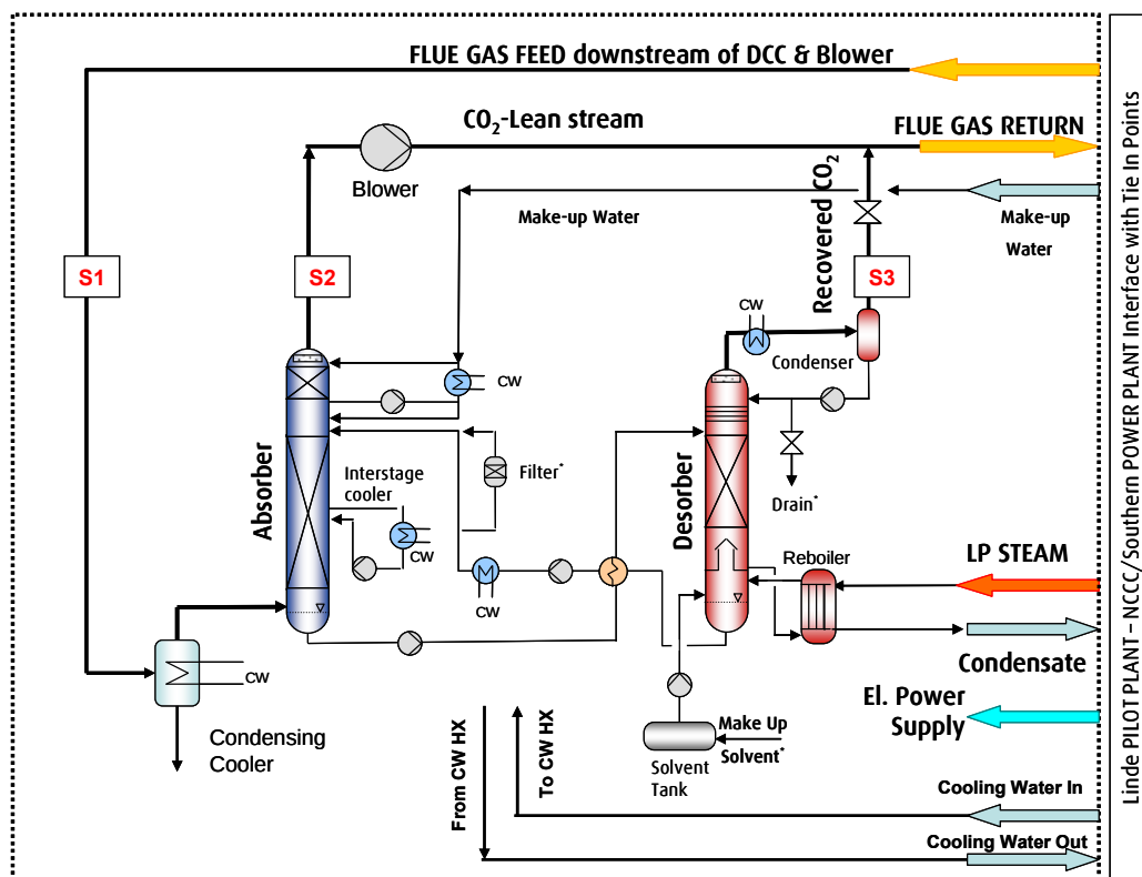
Utilities for 30_TPD Pilot Plant
