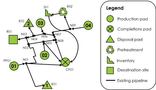
Figure 4. Produced water network case study.
