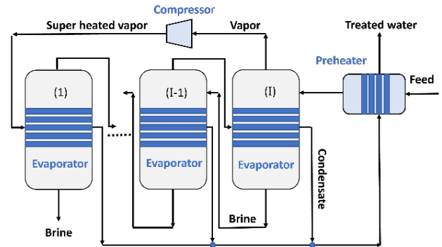
Figure 3. MEE-MVR process with heat integration.
