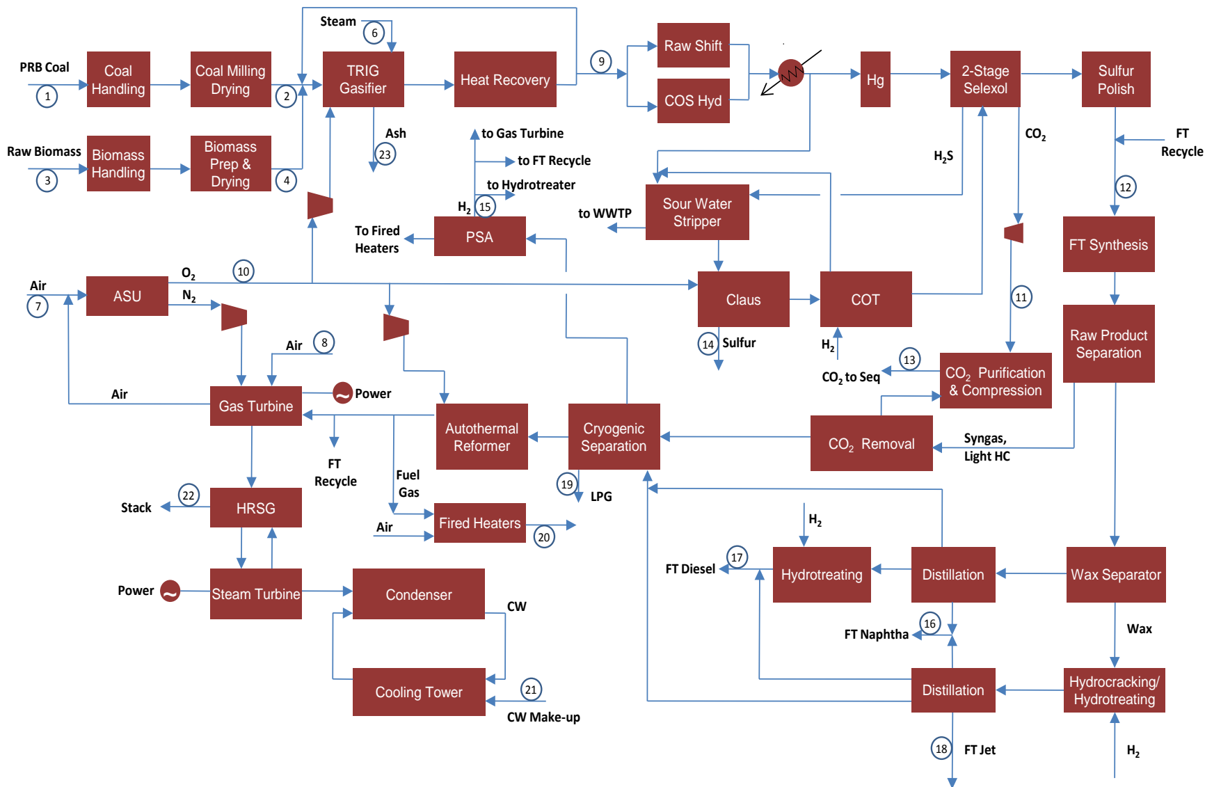
Figure 1: CBTL Facility Configuration: Coal/Green Woody Biomass
