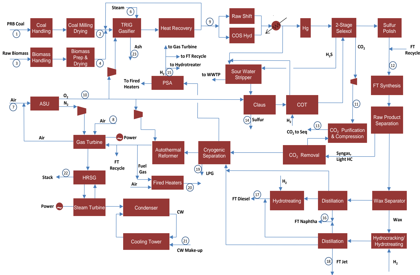
Figure 1: CBTL, 10% Chipped Biomass Facility Configuration
